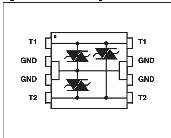
Figure 1. Schematic diagram
